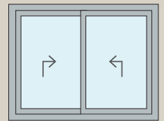
Corredera elevable
